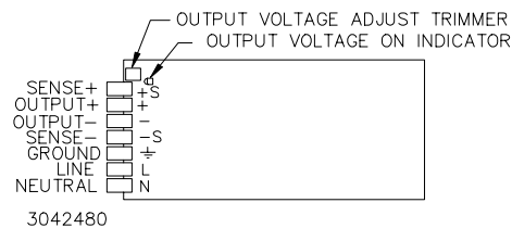
FIGURE 2. COMPONENT LOCATIONS
